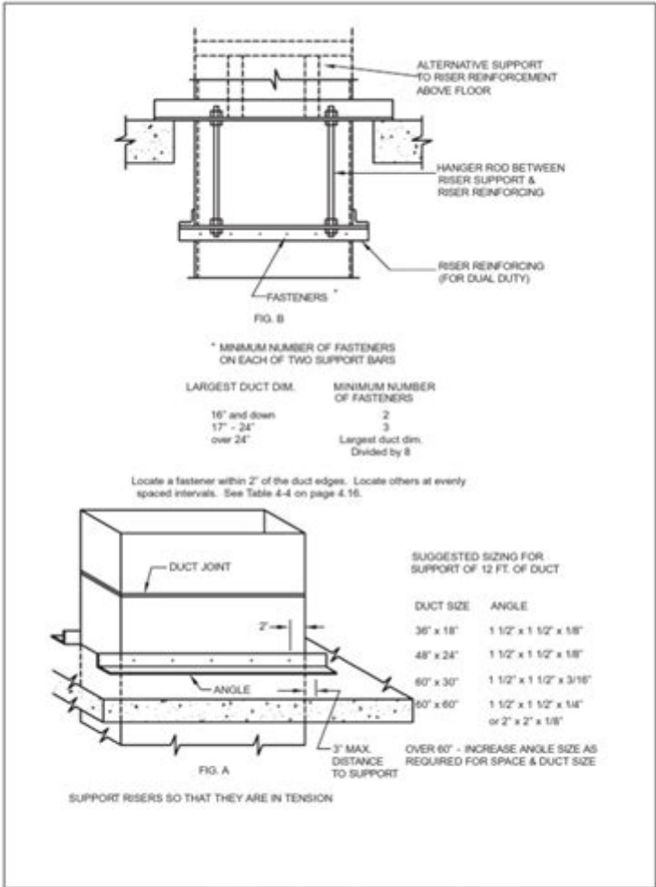
FIGURE 4-7 RISER SUPPORTS - FROM FLOOR
